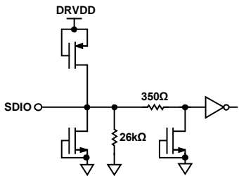
Figure 22. Equivalent SDIO Circuit
