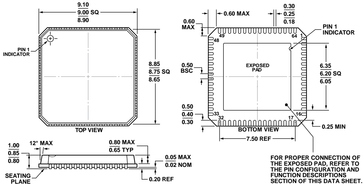
COMPLIANT TO JEDEC STANDARDS MO-220-VMMD-4 Figure 47. 64-Lead Lead Frame Chip Scale Package [LFCSP_VQ] 9 mm × 9 mm Body, Very Thin Quad (CP-64-4) Dimensions shown in millimeters
